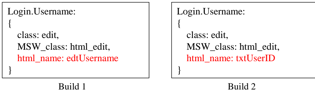
Figure 2. Changes in object property between builds
