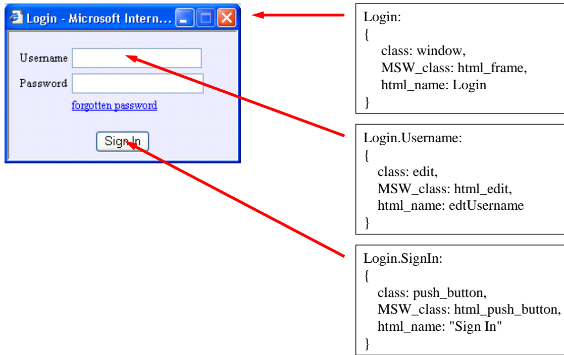
Figure 1. GUI Object Identification
